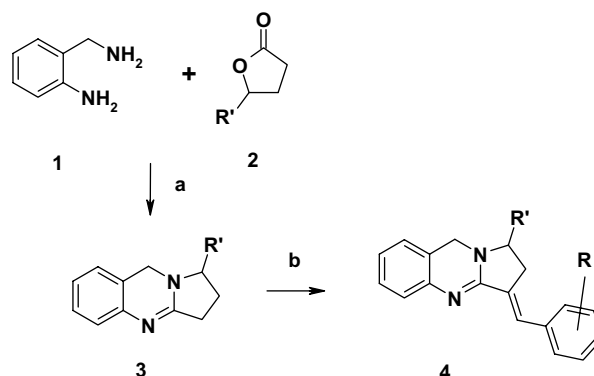
Scheme 1. Synthesis of target compounds 4 . Reagents and conditions: (a) (1) \Delta ; (2) \text{POCl}_3 ; (b) \text{Ar-CHO} , \Delta .
