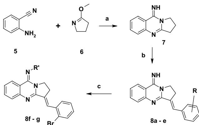
Scheme 2. Synthesis of target compounds 8. Reagents and conditions: (a) \Delta ; (b) Ar-CHO, \Delta ; (c) \text{Me}_3\text{O}^+\text{BF}_4^-/\text{CH}_2\text{Cl}_2 or BrCN/DMF.
