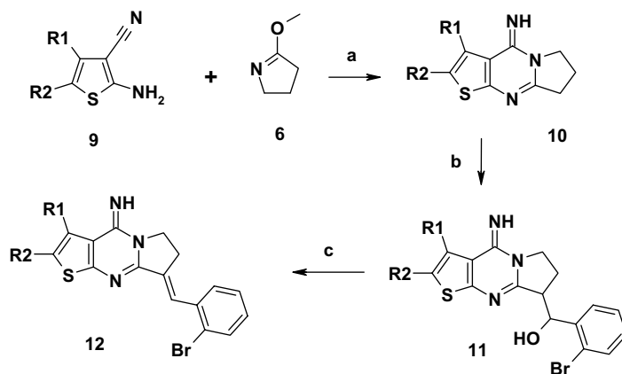
Scheme 3. Synthesis of target compounds 12. Reagents and conditions: (a) \Delta ; (b) o -Br-Ph-CHO, \Delta ; (c) POCl 3 .
